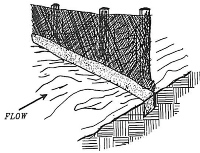
SHEET FLOW INSTALLATION (PERSPECTIVE VIEW)
