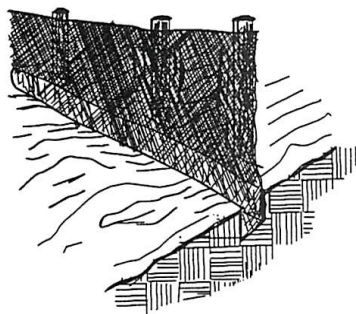
SHEET FLOW INSTALLATION (PERSPECTIVE VIEW)
